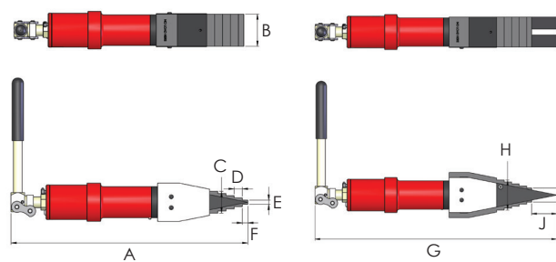
SJS10-M Retracted
