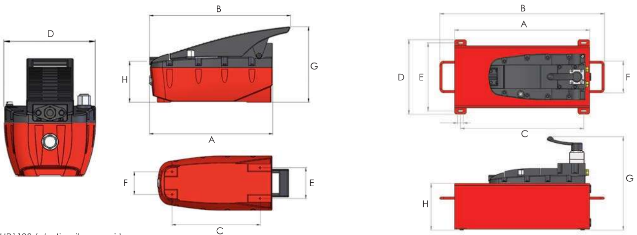
AHP1141 (metal oil reservoir) AHP1142 (metal oil reservoir)
